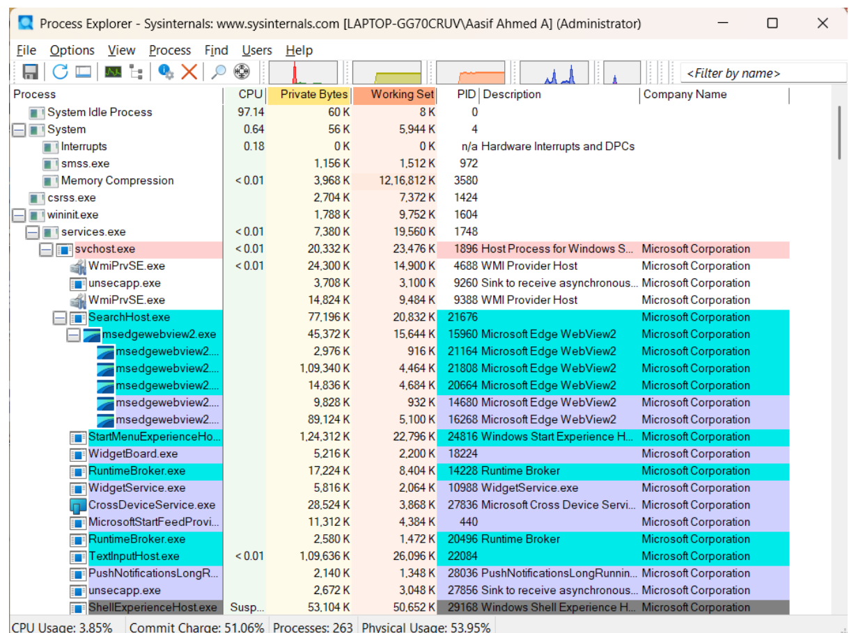
Figure 2: Process Explorer dashboard displaying hierarchical process trees and resource metrics
