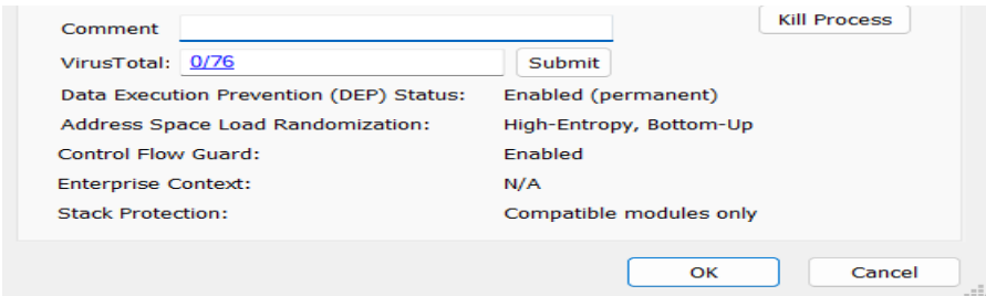
Figure 4: Querying process hashes against online malware repositories
